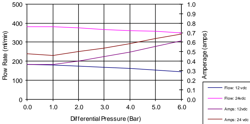
Typical Performance Curve: Water at Room Temperature
